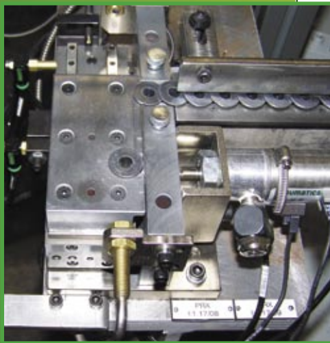
Feeder Escapement, Part Singulation
